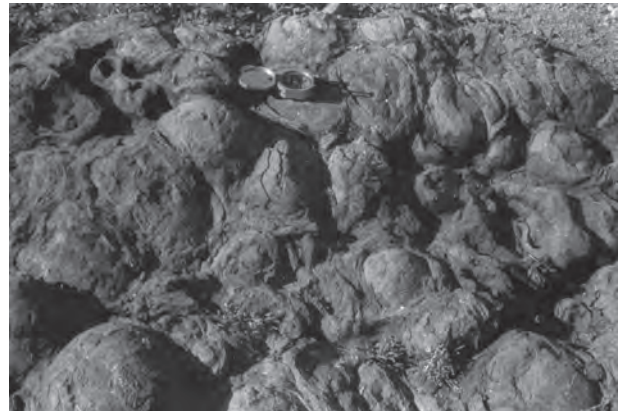
Fig.5.3 : Exfoliation (Flacking) and granular disintegration
