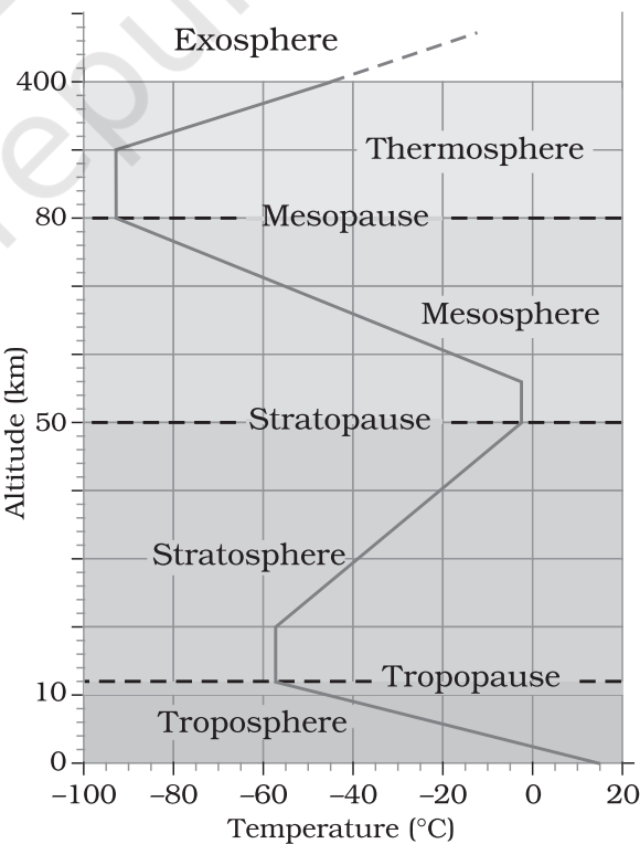
Figure 7.1 : Structure of atmosphere
