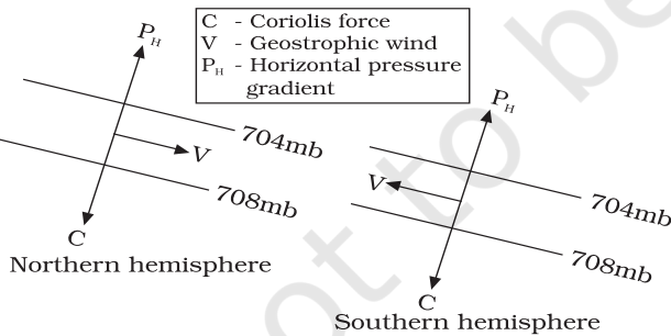
Figure 9.4 : Geostrophic Wind
