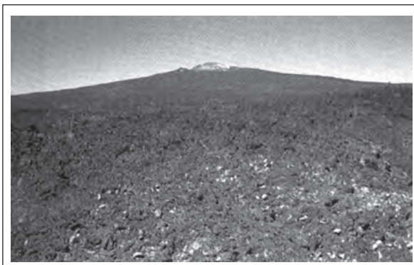
Cinder Cone
